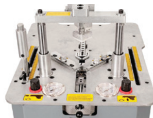
Model UP5-PH, top view
