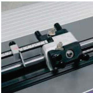
Each cutting head rotates 45° and 90° on two ball bearings. This makes cutting effortless eliminating operator hand and wrist fatigue. The aluminum mat guide, in perfect alignment with the cutting head, ensures an accurate cut on the entire surface of the mat.
