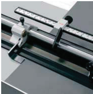
The magnetic stop is a revolutionary feature. Cutting is quicker and more precise. It eliminates the necessity of resetting the opening dimension stops for all 4 sides since the magnets automatically adjust to the external mat size and cuts mats of varying sizes without resetting the stops when you maintain the same border size. The magnetic stops will increase your production.
