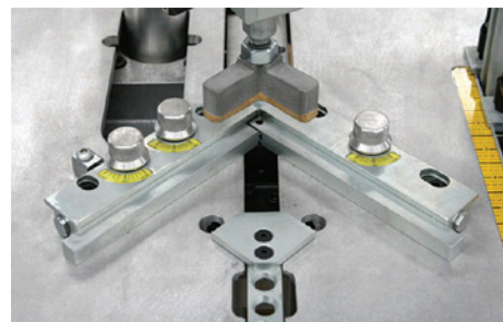
Model UP5-PH, top view
