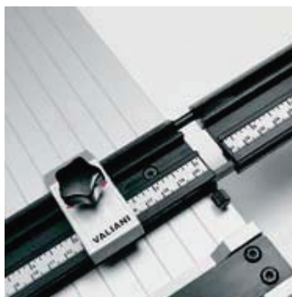
The right side extension arm allows for cuts of up to 120cm (48"). Simple to insert, it provides rigid and stable support for acquiring and cutting to size large mat boards. Includes a measuring stop to help set up the mat dimensions.
